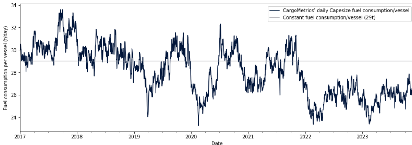
CAPE SIZE FUEL CONSUMPTION PER VESSEL PER DAY, 2017-2023
